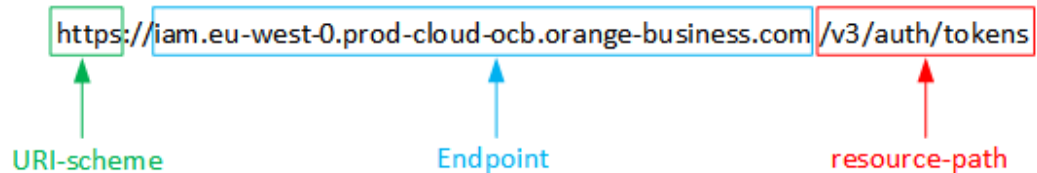
Figure 3-1 Example URI
